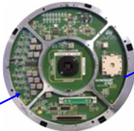
Tester Side
